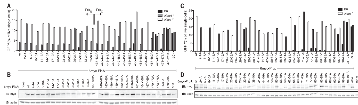
Fig. 4. Multisurface ligand recognition is common to NAIPs. (A) Full-length 6myc-tagged L. pneumophila FlaA, or variants with the indicated residues mutated to alanine, were transduced into BMMs by using a retrovirus marked with IRES (internal ribosomal entry site)–GFP. Transduction efficiency was assessed by flow cytometry for GFP expression at day 4. Failure to transduce B6 BMMs, as compared with transduction of Nlr4 −/− BMMs, is indicative of NAIP activation (5). Naip5 −/− BMM responses to FlaA are
