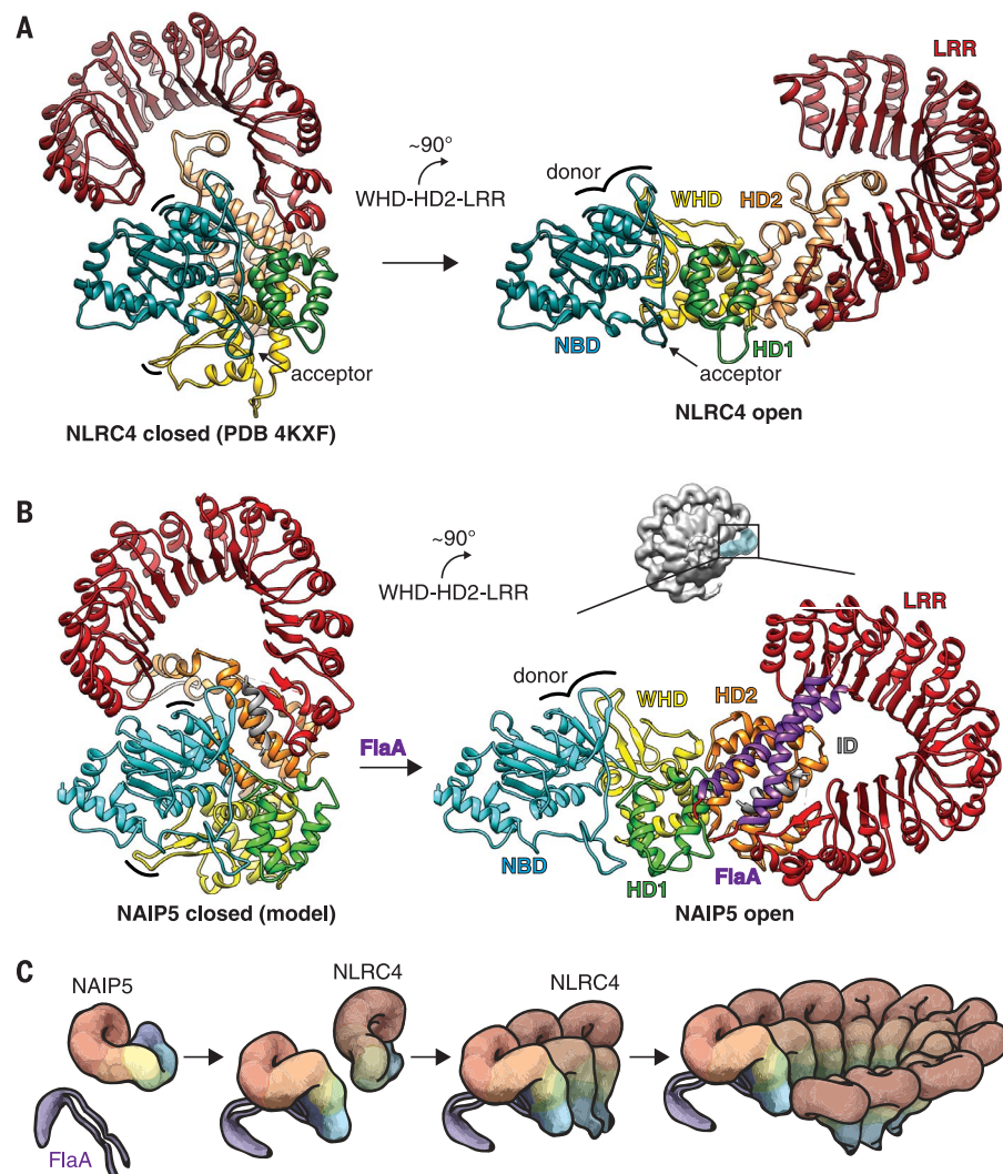
Fig. 3. Model of NAIP5-NLRC4 inflammasome assembly. (A) Structures of inactive (left) and active (right, determined in this work) NLRC4, showing a ~90° rigid-body rotation of the WHD-HD2-LRR module (9, 10) triggered by interaction with an activated NAIP5 or another already activated NLRC4. (B) To generate the inactive NAIP5 conformation [left; modeled based on NLRC4 (methods)], the HD2 insert was moved to avoid collision with the NBD. We propose that flagellin binding induces a ~90° rigid-body rotation of the WHD-HD2-LRR module, analogous to the rotation of NLRC4, which displaces the occluding LRR and HD2 from the NBD to complete and expose the donor oligomerization surface (indicated by curved lines in left and right panels) for interaction with NLRC4. (C) Proposed events of inflammasome assembly. The flagellin D0 domain (purple) binds to NAIP5 and unfurls the protein for subsequent NLRC4 recruitment and activation. Active NLRC4 recruits further NLRC4 protomers for self-propagating oligomerization and completion of a caspase-1 recruitment platform. Colors are as in Fig. 1A.
