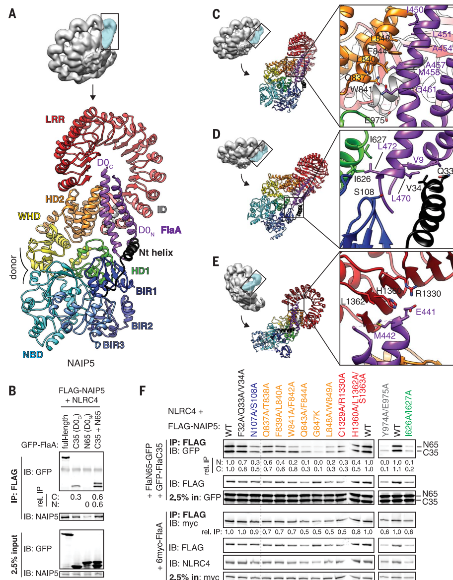
Fig. 2. Multiple NAIP5 domains contact extended surfaces on both helices of the flagellin D0 domain. (A) The D0 domain (purple) is locked into place by multiple NAIP5 domains. (B) Both D0 helices bind to NAIP5. (C to E) Detailed interactions between the flagellin D0 helices and the NAIP5 domains HD2 and ID (C); Nt, BIR1, and HD1 (D); and LRR (E). Side chains shown correspond to mutated residues in (F). (F) Mutagenesis confirms the importance of NAIP5 residues in binding D0 N , D0 C , or full-length FlaA. Point mutations in NAIP5 residues that contact D0 C disrupt both D0 N and D0 C binding because association of D0 N requires D0 C binding [(B) and fig. S9A]. In (B) and (F), relative IP strength was quantified by densitometry [IP signal normalized to input and then GFP-FlaA (B) or WT NAIP5 (F)]. Results are representative of at least three independent experiments. IP, immunoprecipitation; IB, immunoblot; WT, wild type. Single-letter abbreviations for the amino acid residues are as follows: A, Ala; C, Cys; D, Asp; E, Glu; F, Phe; G, Gly; H, His; I, Ile; K, Lys; L, Leu; M, Met; N, Asn; P, Pro; Q, Gln; R, Arg; S, Ser; T, Thr; V, Val; W, Trp; and Y, Tyr.
