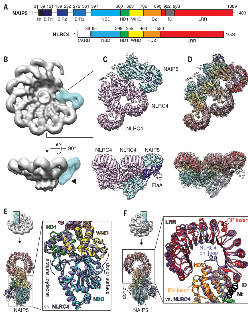
Fig. 1. Structure of the NAIP5-NLRC4 inflammasome. (A) Schematic of domain architecture for NAIP5 and NLRC4. NAIP5 domains were defined in this work (methods); NLRC4 domains were previously defined (19). Residue numbers are shown. Nt, N terminus. (B) 3D reconstruction of inflammasomes containing a single NAIP5-FlaA (blue) and nine NLRC4 protomers (gray). The arrowhead highlights extra density that identified the NAIP5 protomer. (C) Refined 3D reconstruction for NAIP5 and the first two NLRC4 protomers at higher resolution (NAIP5 segmented in blue, the two NLRC4 protomers in pink, and FlaA in purple). (D) Modeled structures of NAIP5 and two NLRC4 protomers, all colored by domains as in (A), fitted within the EM map. In (B) to (D), two orthogonal views are shown. (E and F) The structure of NAIP5 [colored as in (A)] is aligned with that of an NLRC4 protomer (purple). (E) The NBD, HD1, and WHD oligomerization domains of NAIP5 and NLRC4 are highly similar. Oligomerization donor and acceptor surfaces [(9, 10) and fig. S5] are indicated. For clarity, the NAIP5 BIR domains were omitted from the inset view (right). (F) The HD2 and LRR of NAIP5 diverge from those of NLRC4. NAIP5-specific insertions, including an extra leucine-rich repeat (LRR insert; residues 1102 to 1138) and the modeled helix of the inserted domain (ID; gray), are indicated. The NLRC4 S533 phosphorylation loop is replaced by two alpha helices in NAIP5 (HD2 insert; residues 818 to 851).
